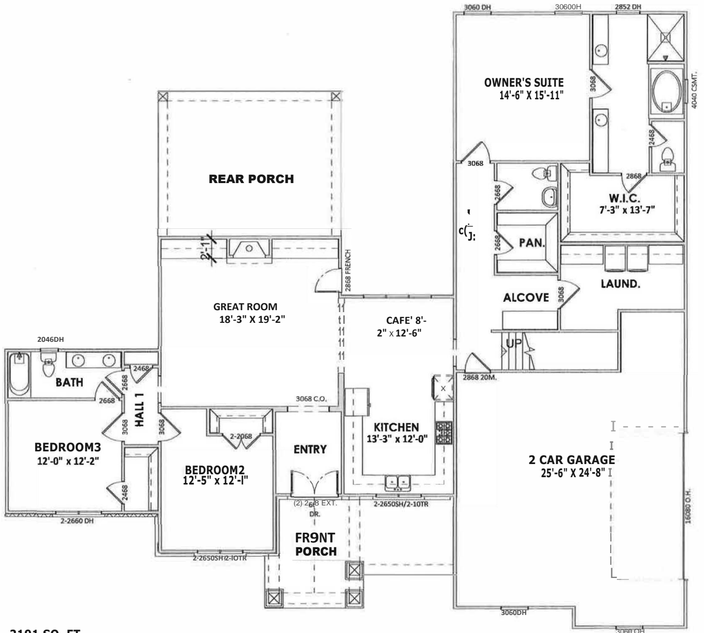
2191 SQ. FT. First Floor Plan- 2 Car Garage
