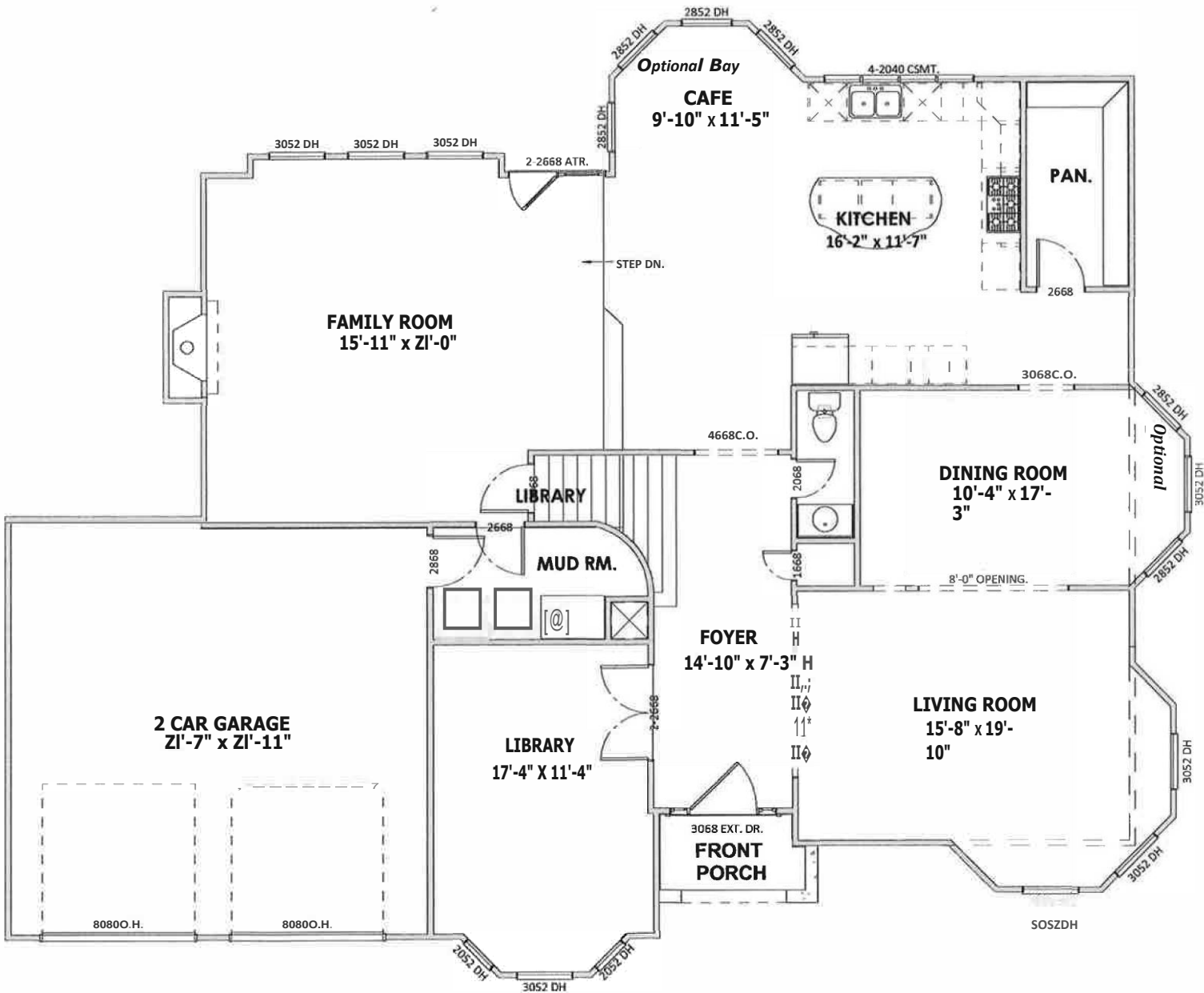
First Floor Plan- 2 Car Garage
